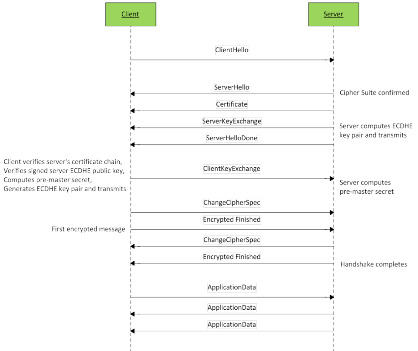
Figure 1: Ephemeral Handshake
