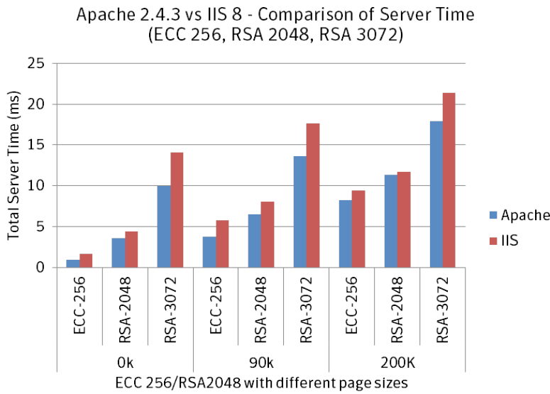
Figure 2: Server Time
